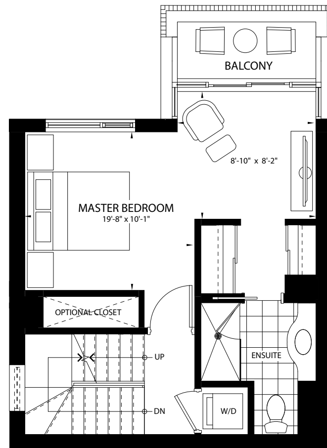
MASTER FLOOR (Standard Second Floor)
